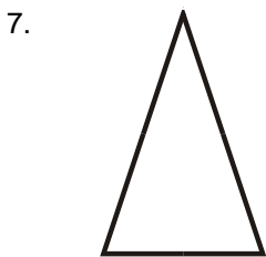
Isosceles Triangle
