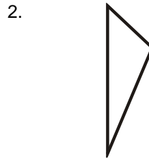
Scalene Triangle
