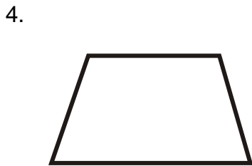
Trapezoid
