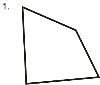
Irregular Quadrilateral
